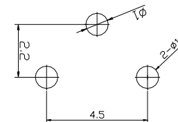
PCB. 焊接图 PCB. WELDING DRAWING
