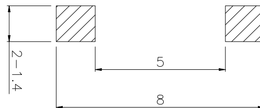
PCB. 焊接图 PCB. WELDING DRAWING
