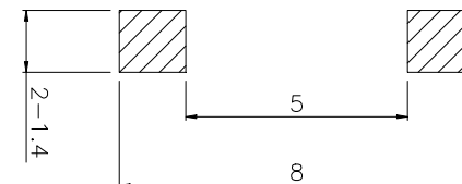
PCB. 焊接图 PCB. WELDING DRAWING
